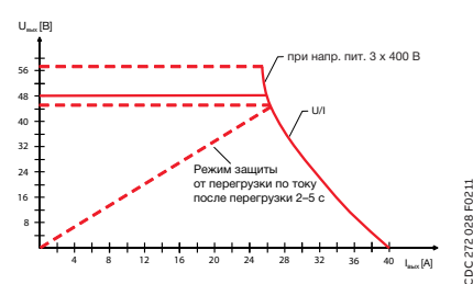
CP-T 48/20.0
