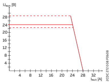
CP-E 24/20.0
