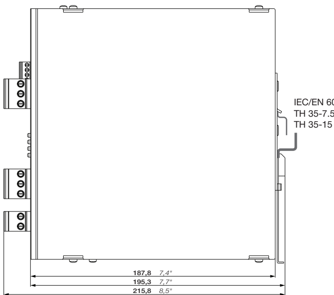
CP-B 24/20.0
