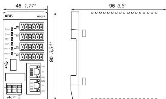
MTQ22 PNQ22
