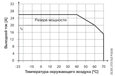
CP-C.1 24/20.0
