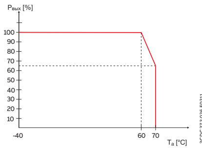
CP-T 24/40.0, CP-T 48/20.0
