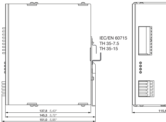
CP-B 24/10.0
