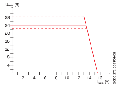
CP-E 24/10.0
