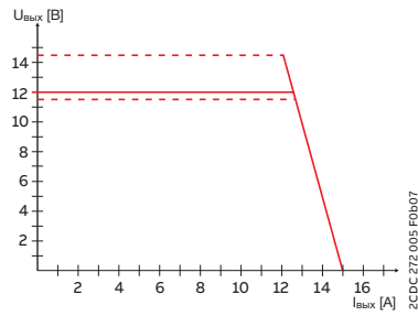
CP-E 12/10.0
