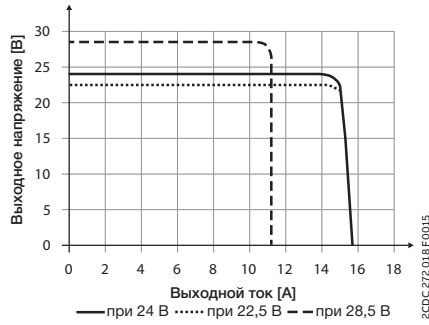
CP-C.1 24/10.0
